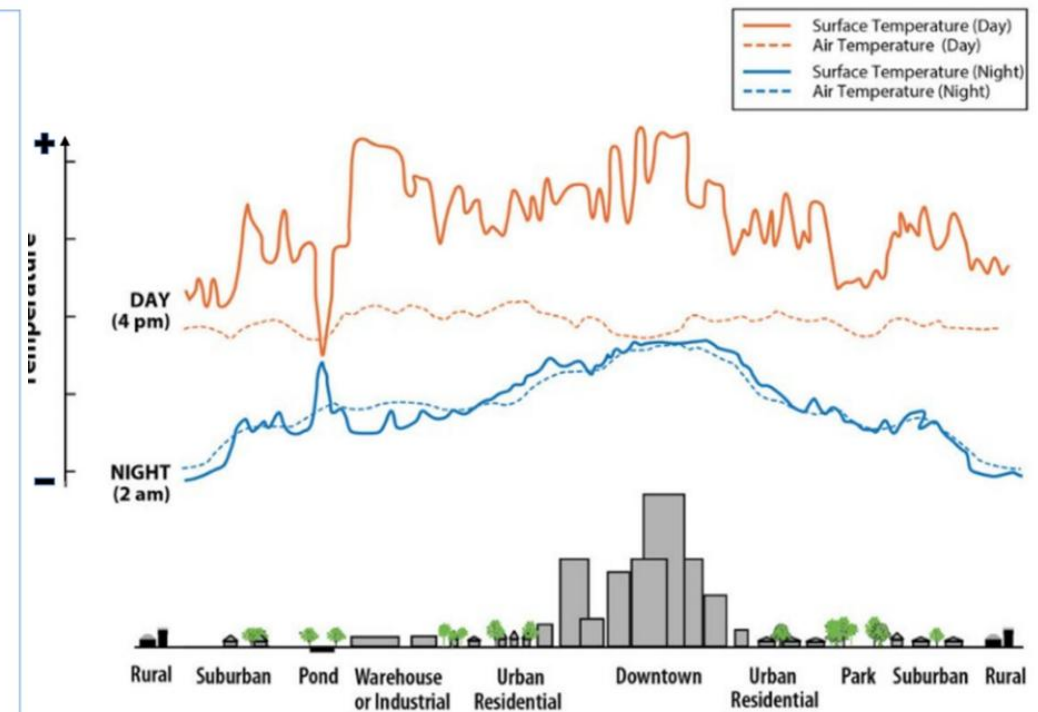
Figure 1. The temperature profile in different areas, with the formation of the UHI (adapted from [3]).
